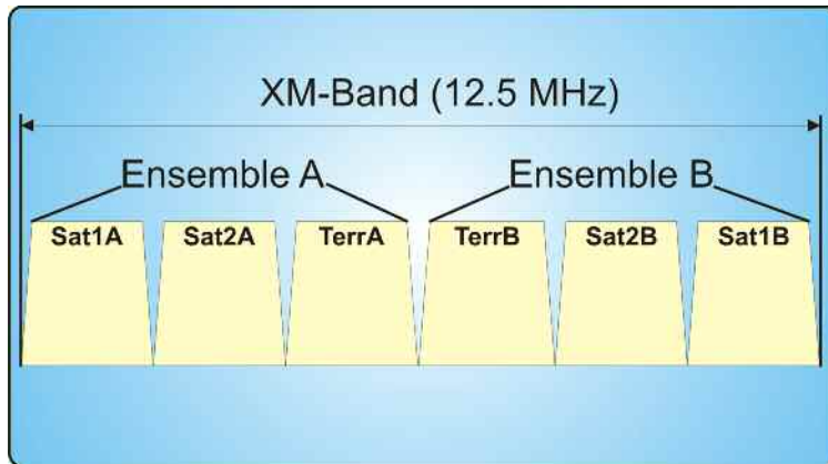
Fig. 1 XM-Radio Frequency Band
